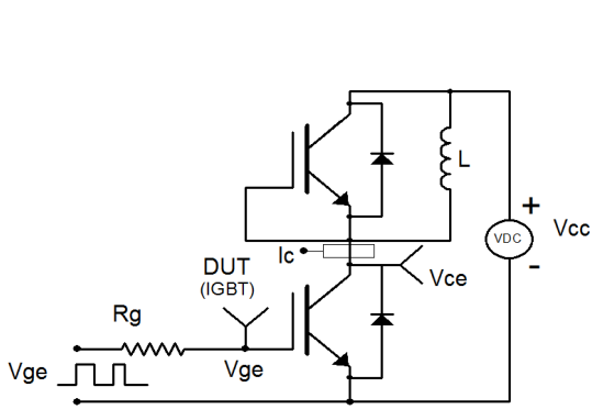
Figure A: Gate Charge Test Circuit & Waveforms
