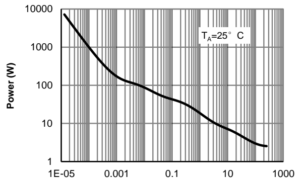
Figure 15: Single Pulse Power Rating Junction-to-Ambient (Note H)
