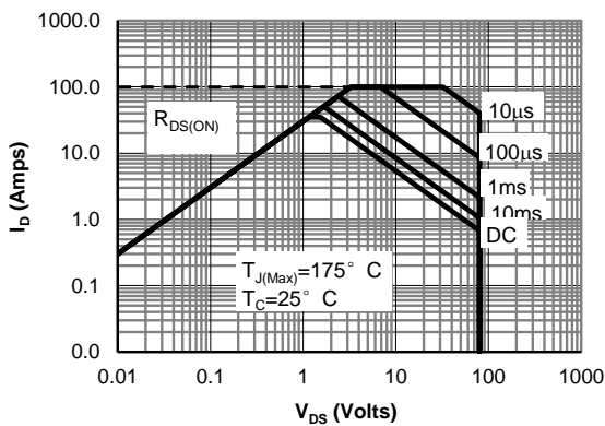
Figure 9: Maximum Forward Biased
