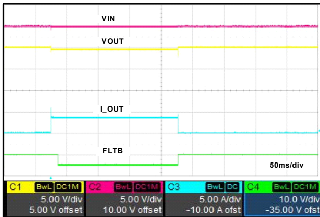
Figure 13. Short Duration Over Current w/o causing Thermal Shutdown (LOAD = 1.2\Omega Applied for 200ms, Device Option -04)
