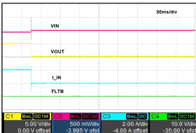
Figure 17. Short Circuit Protection (LOAD = 2.5\Omega , Device Option -04)
