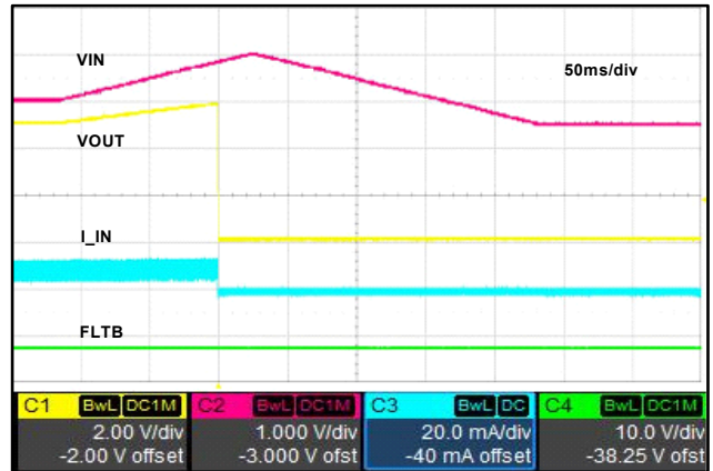
Figure 14. Over-Voltage Protection (LOAD = 938\Omega - Device Option -04)
