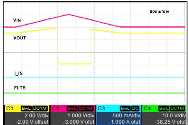
Figure 16. Over-Voltage Protection and Recovery (LOAD = 10\text{k}\Omega , Device Option -03)
