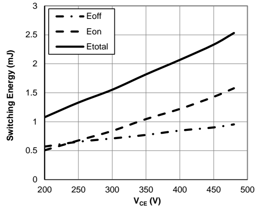
Figure 20: Switching Loss vs. V_{CE} ( T_j=175^\circ C, V_{GE}=15V, I_C=40A, R_g=7.5\Omega )
