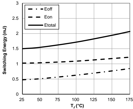
Figure 19: Switching Loss vs. T_j ( V_{GE}=15V, V_{CE}=400V, I_C=40A, R_g=7.5\Omega )
