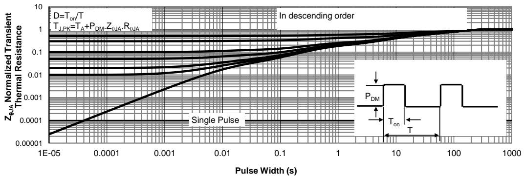
Figure 14: Normalized Maximum Transient Thermal Impedance (Note H)
