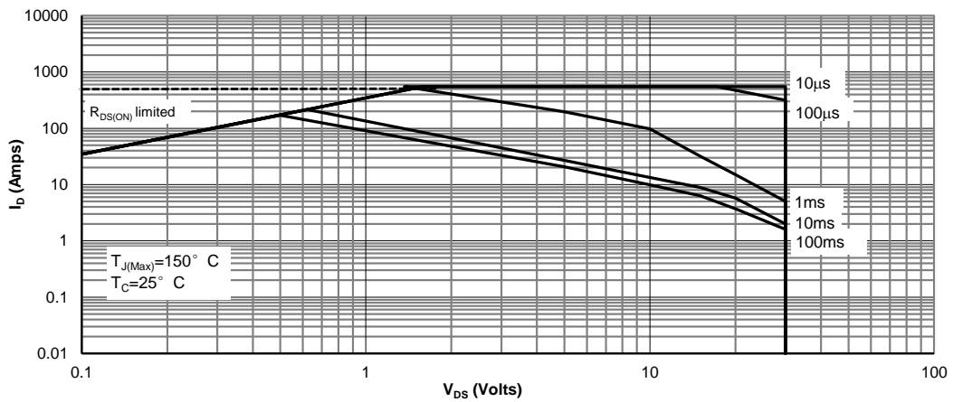
Figure 9: Maximum Forward Biased Safe Operating Area (Note F)
