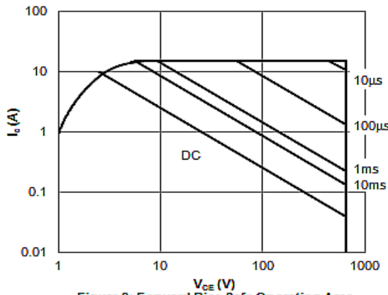
Figure 9: Forward Bias Safe Operating Area ( T_C=25^\circ\text{C} , V_{BE}=15\text{V} )
