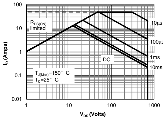
Figure 11: Maximum Forward Biased Safe Operating Area for AOW360A70 (Note F)
