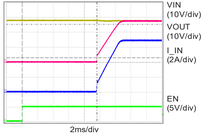
Soft Start Delay Time ( V_{IN} = 28\text{ V} , R_{OUT} = 4\text{ }\Omega )
