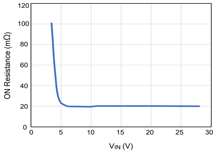
Figure 5. On Resistance vs. VIN
