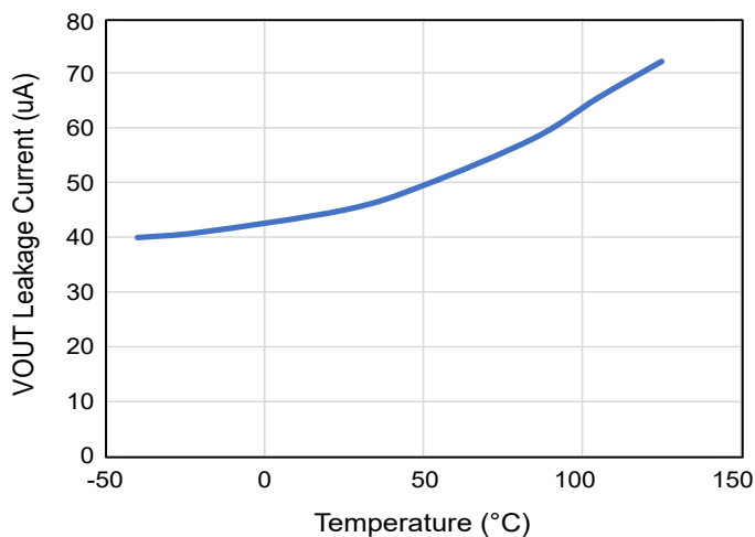
Figure 7. V OUT Leakage Current vs. Temperature
