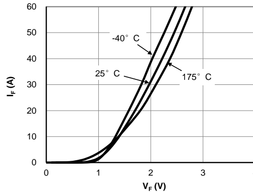
Figure 4: Diode Characteristic
