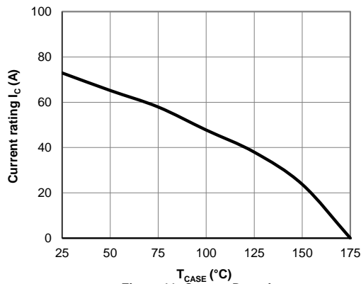
Figure 11: Current De-rating
