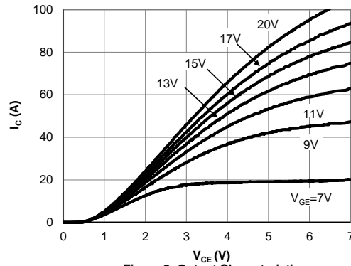
Figure 2: Output Characteristic (T j =150°C)
