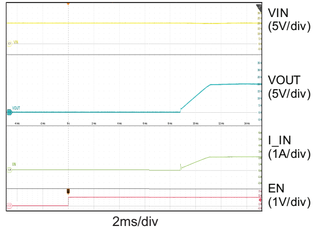
Figure 4. Soft-Start Delay ( V_{IN} = 20\text{V} , R_{OUT} = 9.06\Omega )
