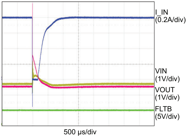
Figure 9. Ideal Diode True Reverse Current Blocking ( R_{OUT} = 20\ \Omega )
