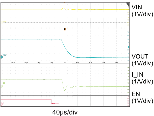
Figure 7. Shutdown ( V_{IN} = 5\text{V} , R_{OUT} = 2.2\Omega )
