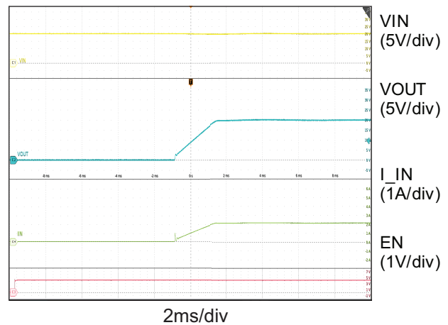
Figure 6. Soft-Start Ramp ( V_{IN} = 20\text{V} , R_{OUT} = 9.06\Omega )
