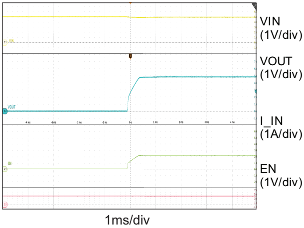
Figure 5. Soft-Start Ramp ( V_{IN} = 5\text{V} , R_{OUT} = 2.2\Omega )
