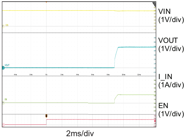
Figure 3. Soft-Start Delay ( V_{IN} = 5\text{V} , R_{OUT} = 2.2\Omega )
