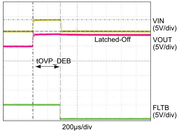
Figure 10. Over-Voltage Protection
