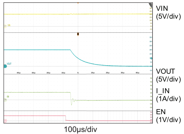
Figure 8. Shutdown ( V_{IN} = 20\text{V} , R_{OUT} = 9.06\Omega )
