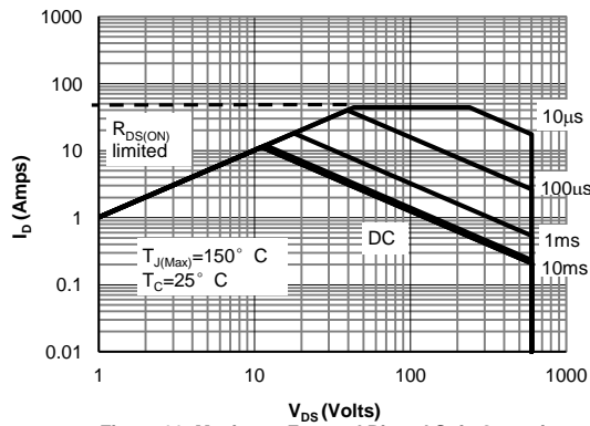
Figure 11: Maximum Forward Biased Safe Operating Area for AOD380A60C (Note F)
