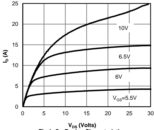
Fig 1: On-Region Characteristics
