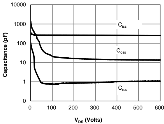
Figure 9: Capacitance Characteristics
