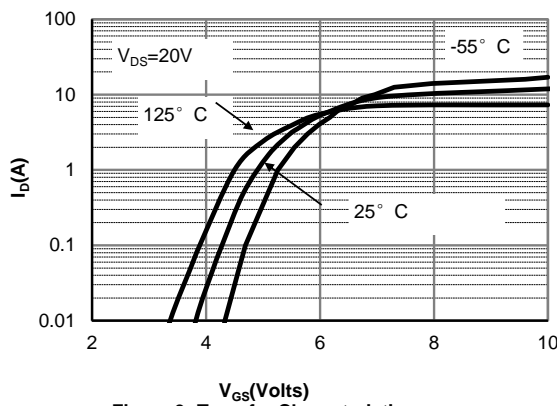
Figure 3: Transfer Characteristics
