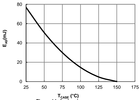
Figure 14: Avalanche energy
