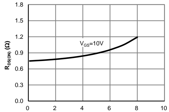
Figure 4: On-Resistance vs. Drain Current and Gate Voltage
