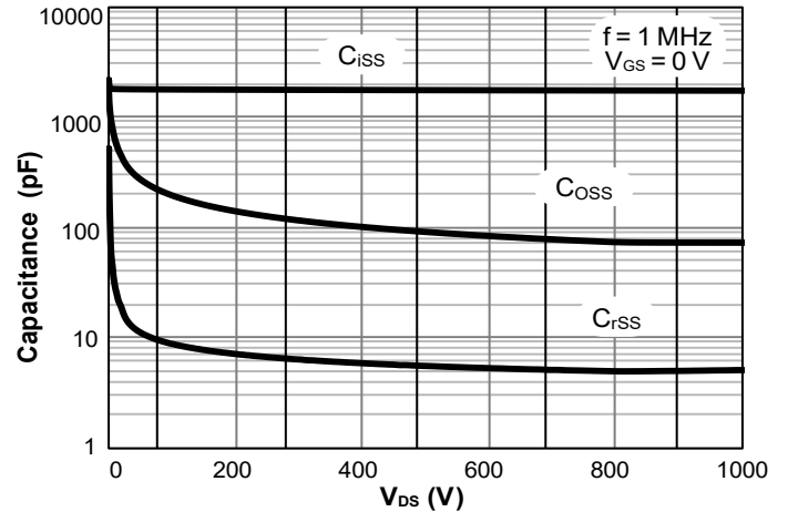
Figure 10. Capacitance Characteristics
