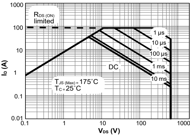
Figure 17. Maximum Forward Biased Safe Operating Area for AOM065V120X2 (Note I)
