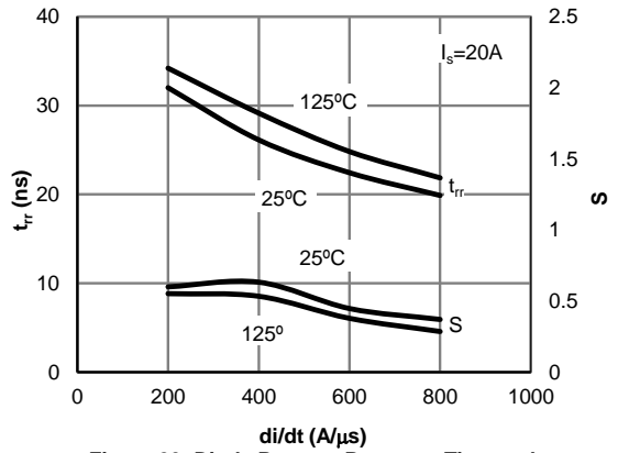
Figure 20: Diode Reverse Recovery Time and Softness Factor vs. di/dt
