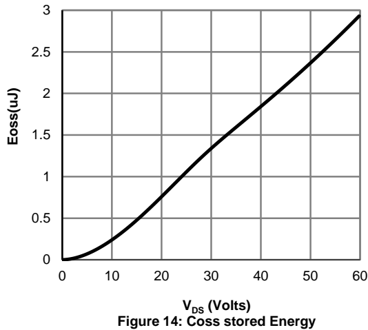
Figure 14: Coss stored Energy
