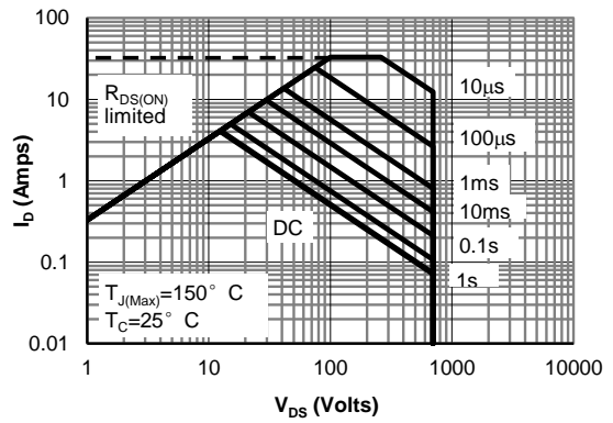
Figure 10: Maximum Forward Biased Safe Operating Area for AOTF9N70 (Note F)
