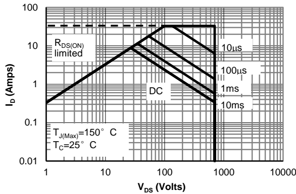
Figure 9: Maximum Forward Biased Safe Operating Area for AOT(B)9N70 (Note F)
