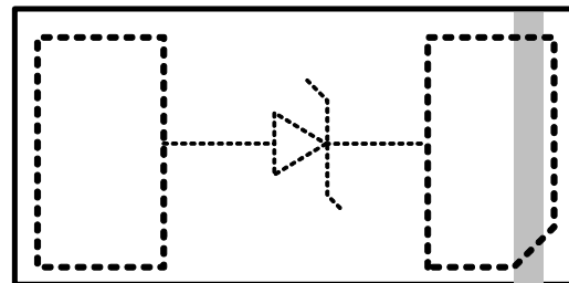
DFN2.0x1.25A_2L
