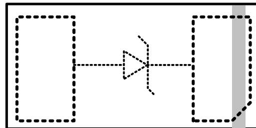
DFN2.0x1.25A_2L
