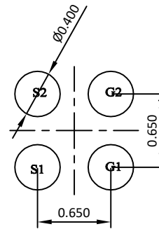
RECOMMENDED LAND PATTERN
