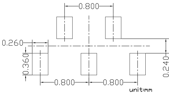
RECOMMEND LAND PATTERN
