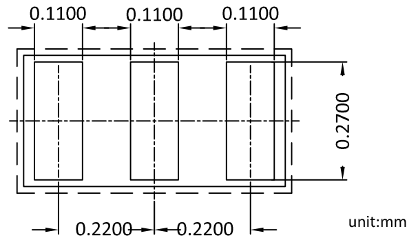
RECOMMEND LAND PATTERN
