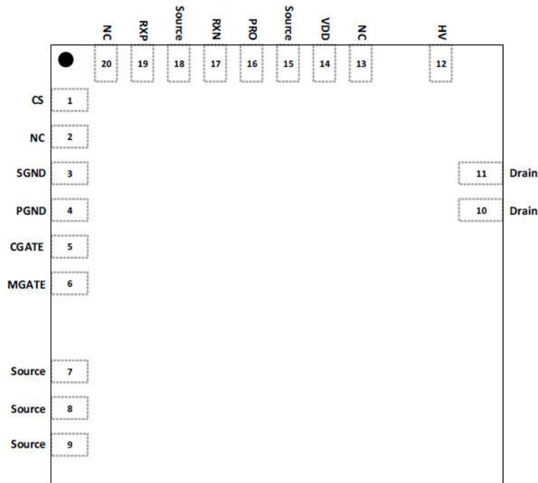
20-Pin 7mm x 7mm QFN (Top View)
