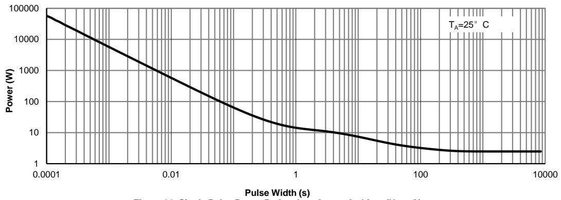
Figure 14: Single Pulse Power Rating Junction-to-Ambient (Note G)
