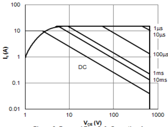
Figure 9: Forward Bias Safe Operating Area ( T_c=25^\circ C, V_{GS}=15V )
