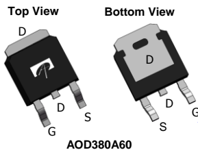
TO252
