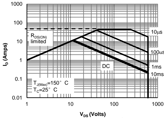
Figure 11: Maximum Forward Biased Safe Operating Area for AOD380A60 (Note F)
