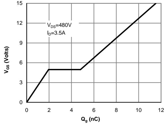
Figure 8: Gate-Charge Characteristics
