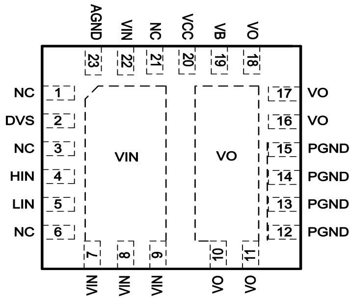
AOZ9511QV
