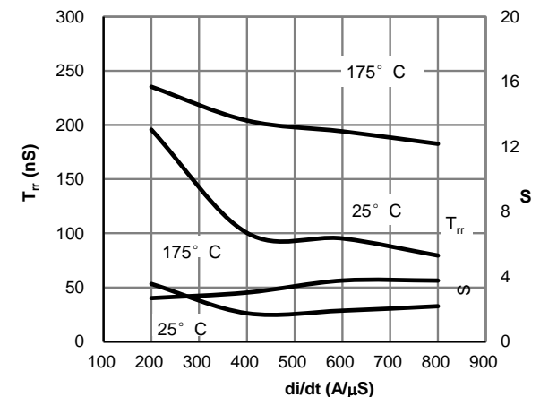
Figure 26: Diode Reverse Recovery Time and Softness Factor vs. di/dt ( V_{GE}=15V, V_{CE}=400V, I_F=15A )
