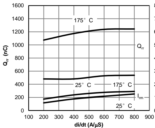
Figure 25: Diode Reverse Recovery Charge and Peak Current vs. di/dt ( V_{GE}=15V, V_{CE}=400V, I_F=15A )
