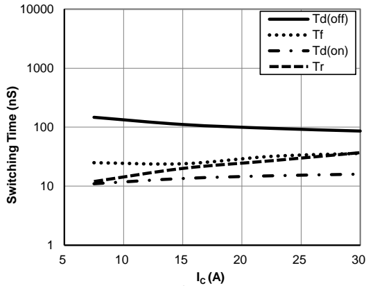
Figure 13: Switching Time vs. I_C ( T_J=150^{\circ}C, V_{GE}=15V, V_{CE}=400V, R_g=20\Omega )
