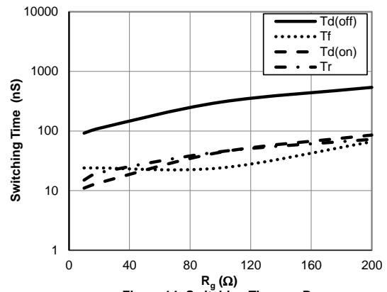
Figure 14: Switching Time vs. R_g ( T_J=150^{\circ}C, V_{GE}=15V, V_{CE}=400V, I_C=15A )
