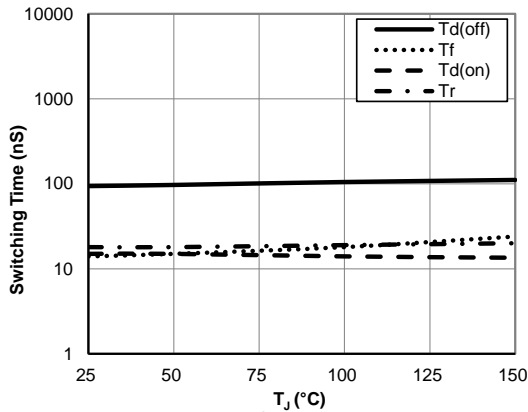
Figure 15: Switching Time vs. T_J ( V_{GE}=15V, V_{CE}=400V, I_C=15A, R_g=20\Omega )
