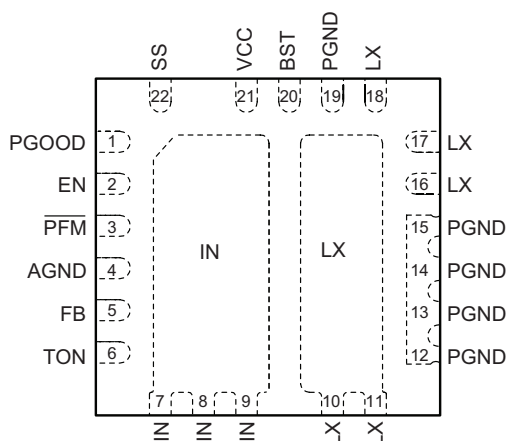
22-Pin 4mm x 4mm QFN (Top View)
