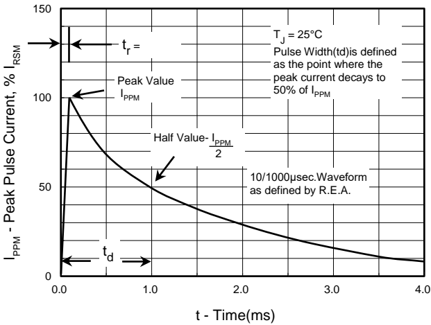
Pulse Waveform
