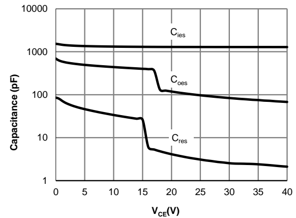
Fig 8: Capacitance Characteristic
