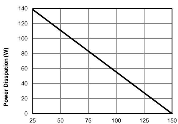
Fig 11: Power Dissipation as a Function of Case
