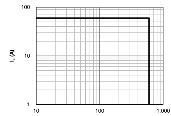
Fig 10: Reverse Bias SOA ( T_J=150^\circ\text{C}, V_{GE}=15\text{V} )
