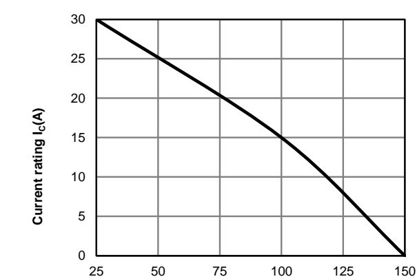
Fig 12: Current De-rating
