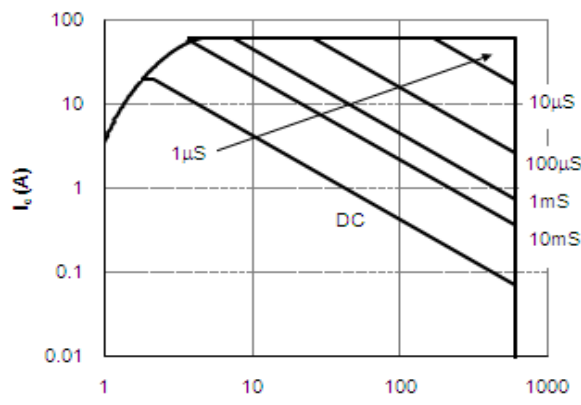
Fig 9: Forward Bias Safe Operating Area ( T_C=25^\circ\text{C}, V_{GE}=15\text{V} )
