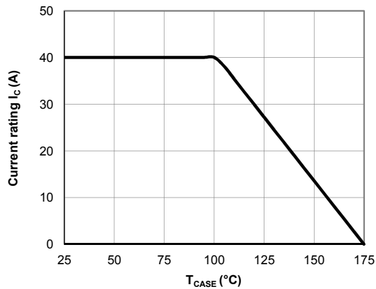
Figure 11: Current De-rating
