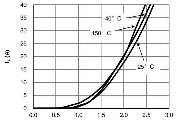
Fig 4: Diode Characteristic
