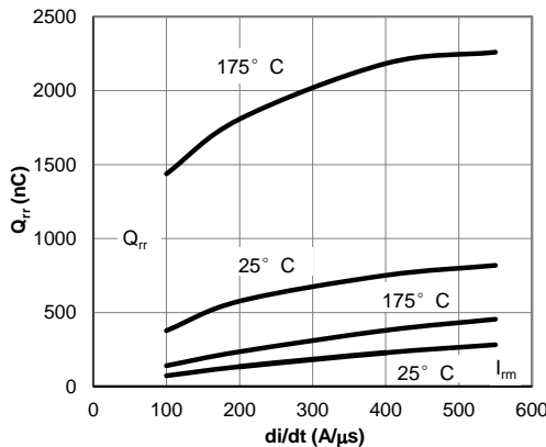
Figure 7: Diode Reverse Recovery Charge and Peak Current vs. di/dt ( V_{GE}=15V, V_{CE}=400V, I_F=40A )
