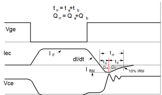
Figure C: Diode Recovery Test Circuit & Waveforms
