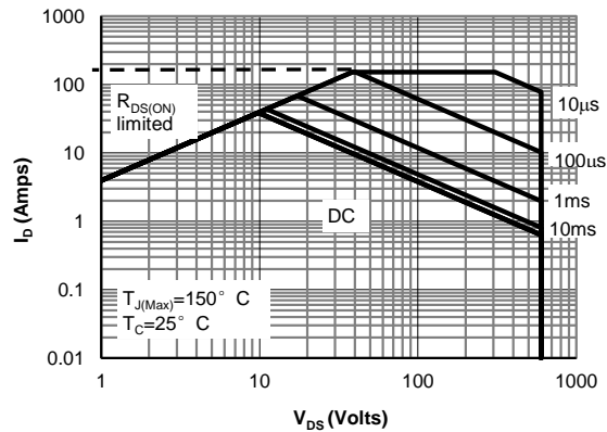
Figure 11: Maximum Forward Biased Safe Operating Area for AOK095A60 (Note F)
