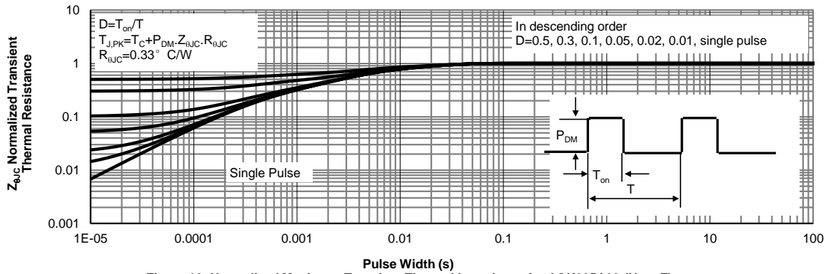
Figure 12: Normalized Maximum Transient Thermal Impedance for AOK095A60 (Note F)
