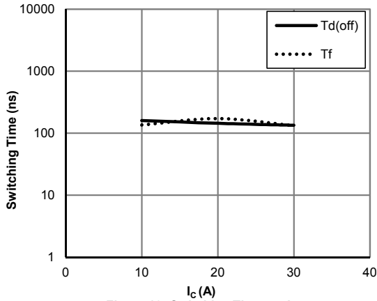
Figure 12: Switching Time vs. I_c ( T_j=175^\circ\text{C} , V_{GE}=15\text{V} , V_{CE}=600\text{V} , R_g=15\Omega )
