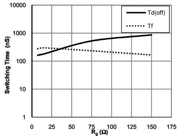
Figure 13: Switching Time vs. R_g ( T_J=175^\circ\text{C}, V_{GE}=15\text{V}, V_{CE}=600\text{V}, I_c=20\text{A} )
