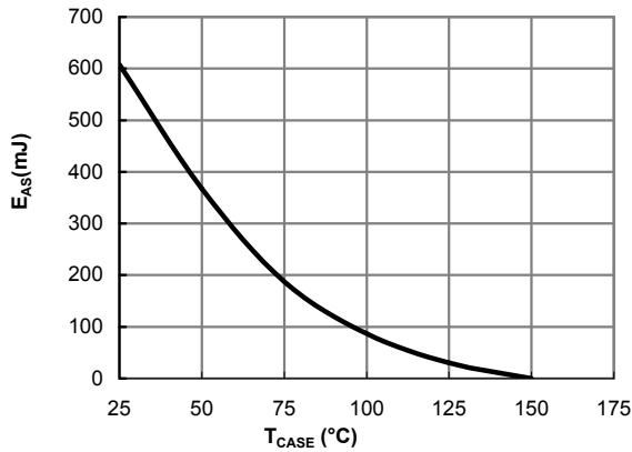
Figure 12: Avalanche energy
