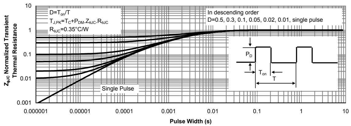
Figure 14: Normalized Maximum Transient Thermal Impedance for AOK29S50 (Note F)
