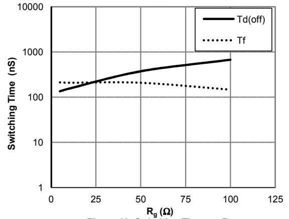
Figure 13: Switching Time vs. R_g ( T_J=175^\circ\text{C}, V_{GE}=15\text{V}, V_{CE}=600\text{V}, I_C=30\text{A} )
