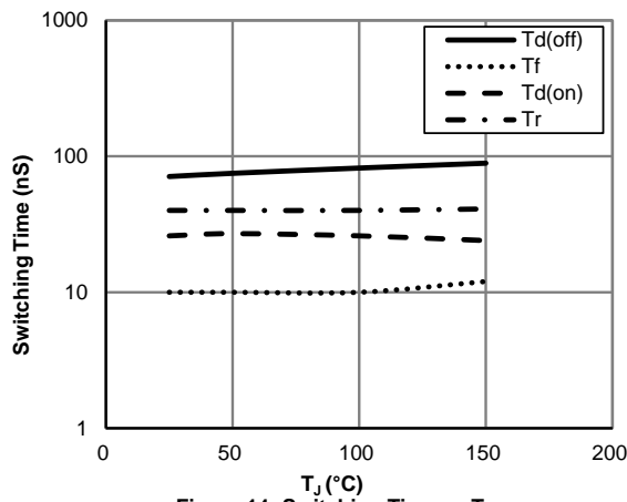
Figure 14: Switching Time vs. T_J ( V_{GE}=15\text{V}, V_{CE}=400\text{V}, I_C=30\text{A}, R_g=10\Omega )
