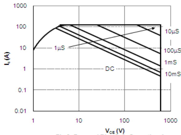
Fig 9: Forward Bias Safe Operating Area ( T_c=25^\circ\text{C}, V_{GE}=15\text{V} )
