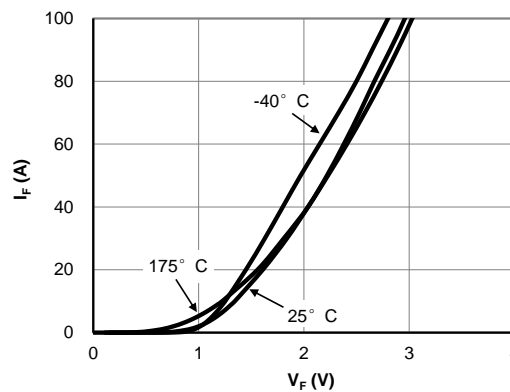
Figure 4: Diode Characteristic
