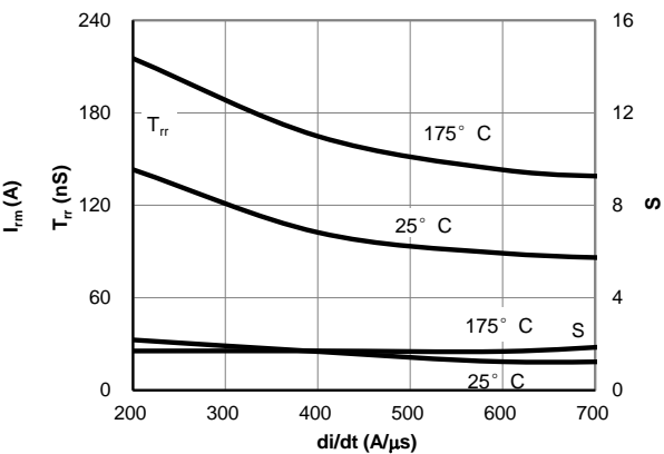
Figure 24: Diode Reverse Recovery Time and Softness Factor vs. di/dt ( V_{GE}=15V , V_{CE}=400V , I_F=30A )
