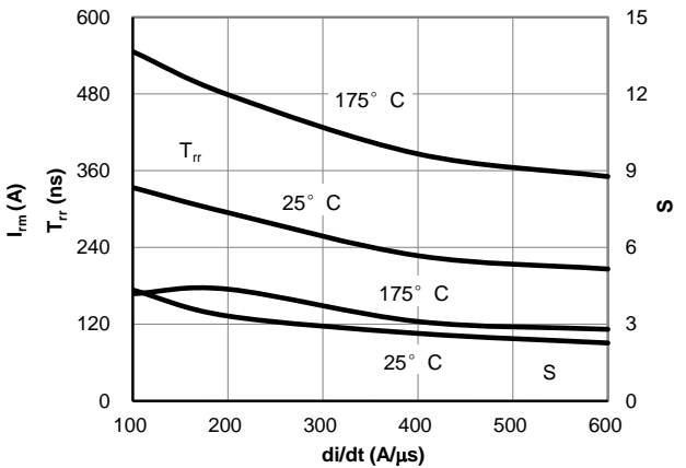
Figure 24: Diode Reverse Recovery Time and Softness Factor vs. di/dt ( V_{GE}=15V , V_{CE}=400V , I_F=75A )
