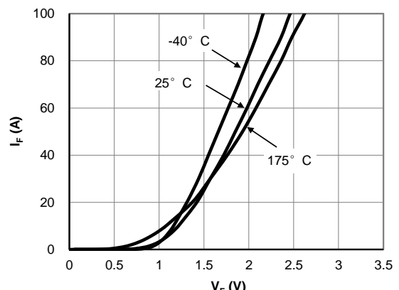
Figure 4: Diode Characteristic
