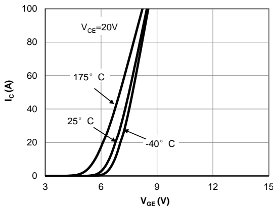
Figure 3: Transfer Characteristic
