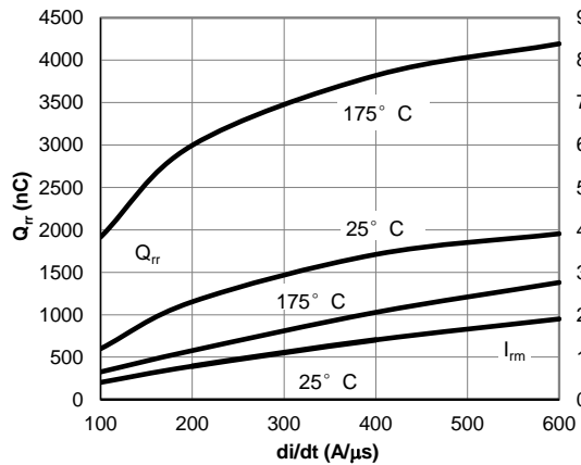
Figure 23: Diode Reverse Recovery Charge and Peak Current vs. di/dt ( V_{GE}=15V , V_{CE}=400V , I_F=75A )
