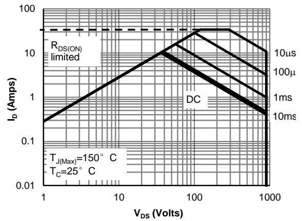
Figure 10: Maximum Forward Biased Safe Operating Area for AOK9N90 (Note F)
