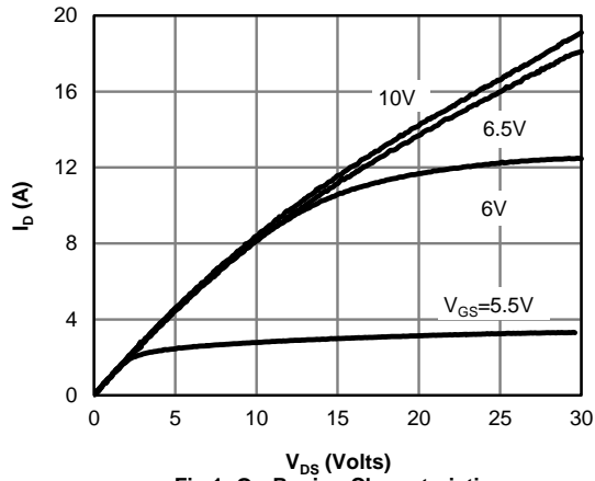
Fig 1: On-Region Characteristics
