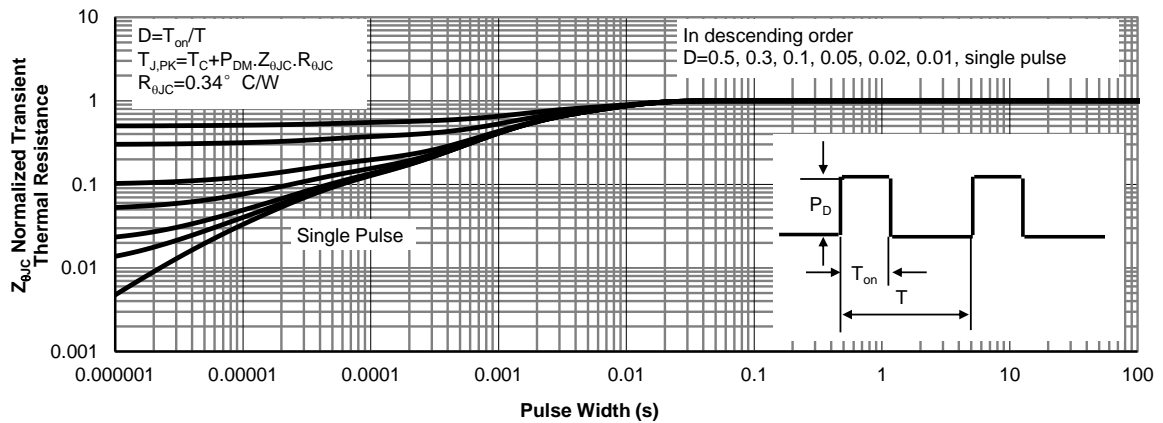
Figure 11: Normalized Maximum Transient Thermal Impedance for AOK9N90 (Note F)
