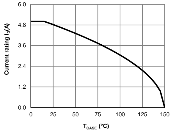
Figure 10: Current De-rating (Note B)
