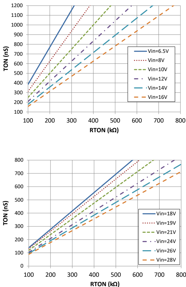
Figure 3. T_{ON} vs. R_{TON} Curves for AOZ1266AQI
