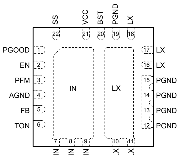
22-Pin 4mm x 4mm QFN (Top View)
